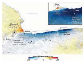
Ground displacement was especially intense near Caracas and La Guaira, Venezuela, after the June 24, 2025 earthquakes. Courtesy of NASA Earth Observatory/Lauren Daughin
